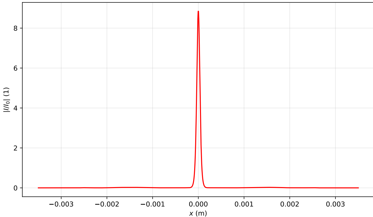
Intensity profile I(x, y = 0, z = 1.115)/I_0 , P_{in}=6.0P_{cr} , artificial time
